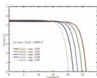
I-V Curves of SPP105QH36S at different cell temperature
